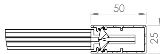
DETAIL K SCALE 1 : 2
